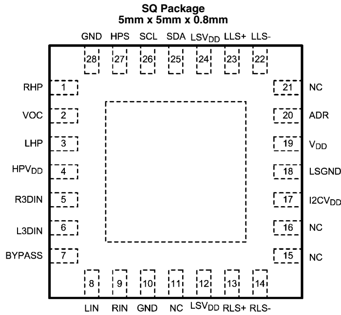
Top View Order Number LM49270SQ See NS Package Number NSQAQ028
